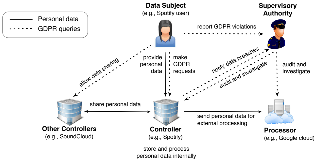
Figure 1: Flow of personal data and GDPR queries between the four GDPR entities: data subjects, data controllers, data processors, and regulators.
